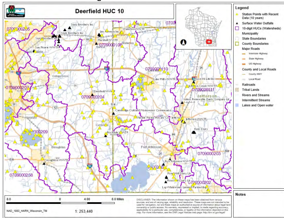
Figure 2-1: HUC 10 Watershed
