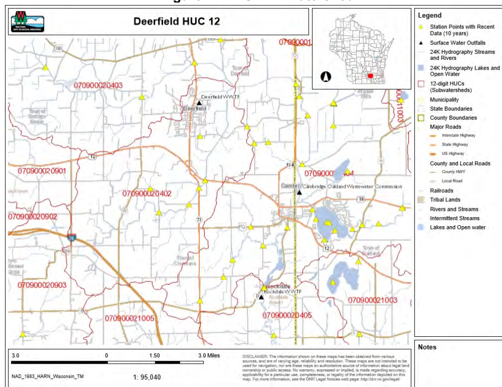
Figure 2-2: HUC 12 Watershed
